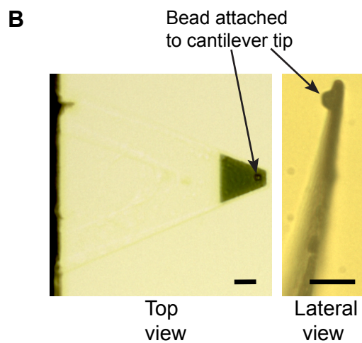
Step 5: Retract the cantilever. Check for the attached bead. Store at RT for overnight.
