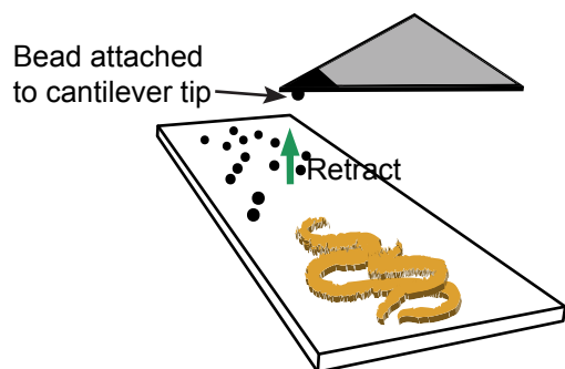
Step 5: Retract the cantilever. Check for the attached bead. Store at RT for overnight.
